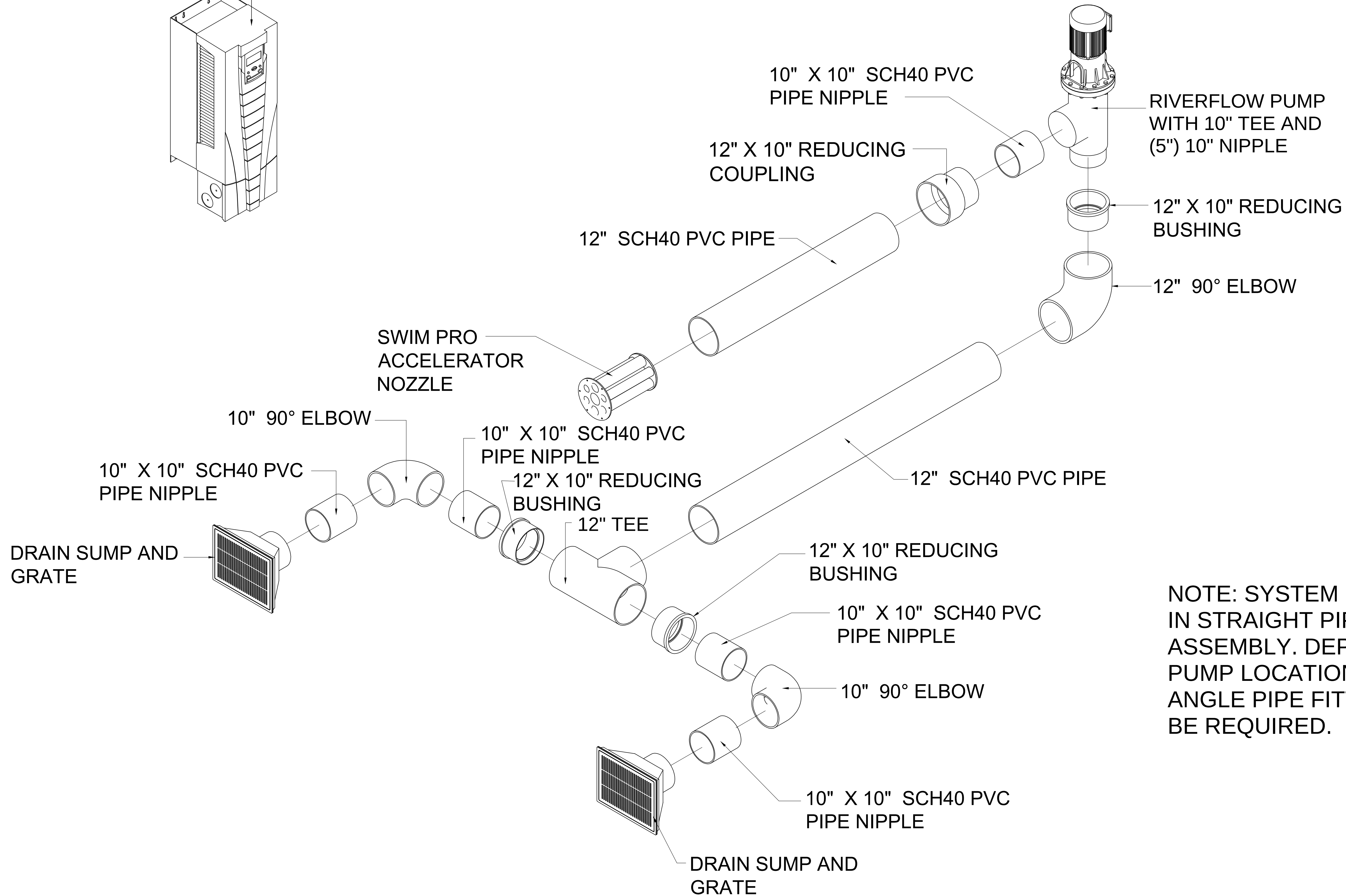
SWIM POOL SYSTEM 10" X 10" SUCTION PORTS (EXPLODED VIEW)
