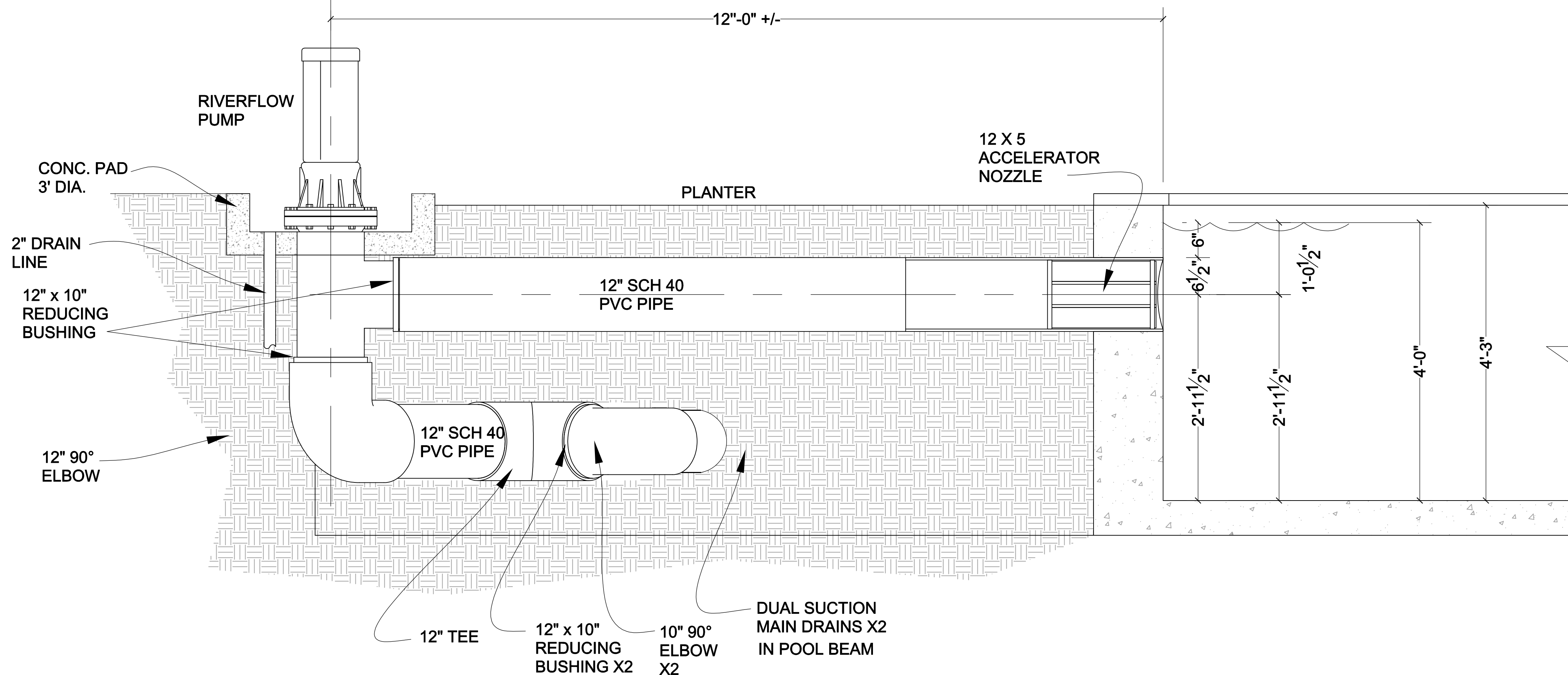
B 2 RIVERFLOW SYSTEM SECTION DETAIL
