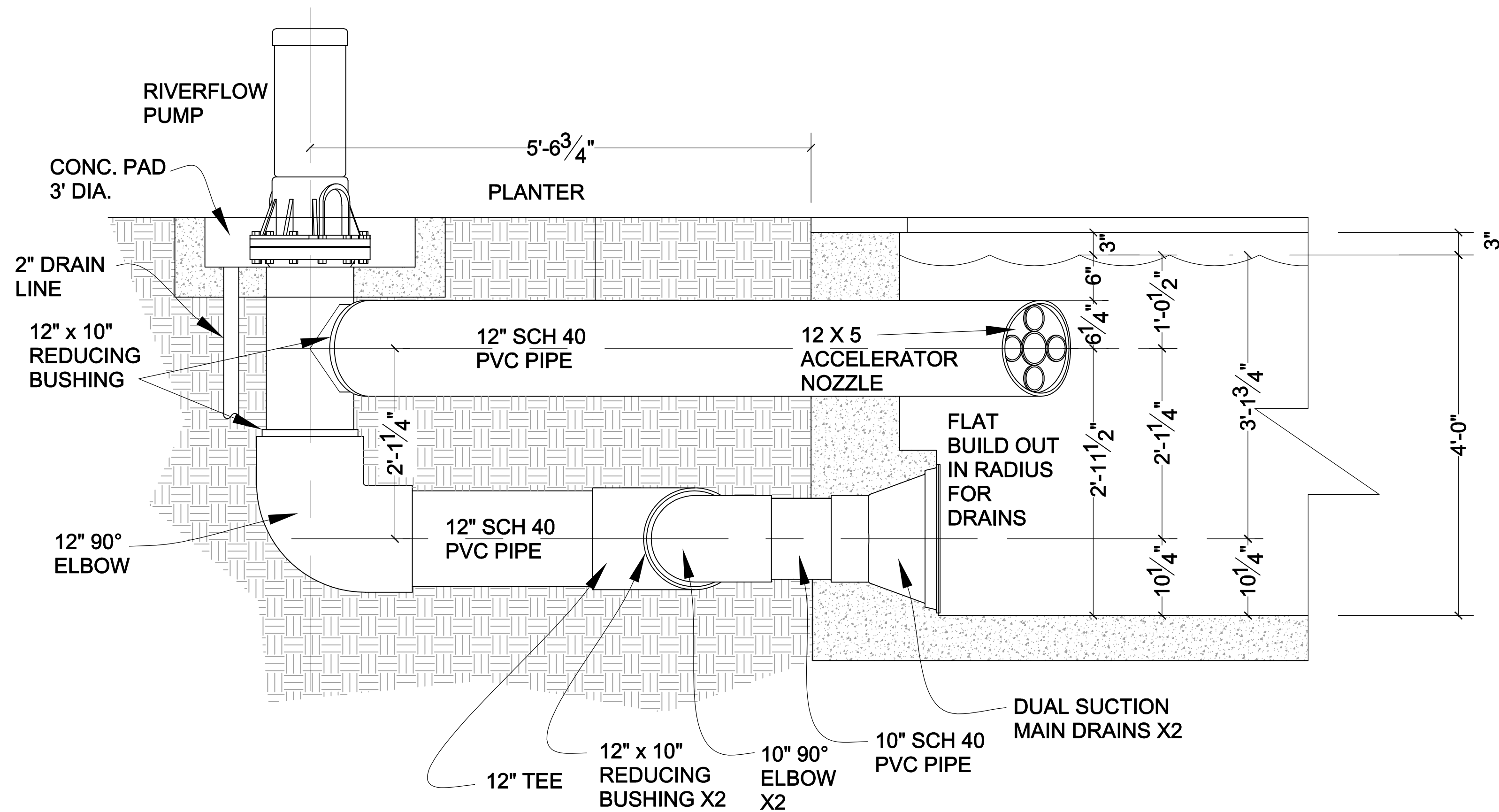
A 2 RIVERFLOW SYSTEM SECTION DETAIL
